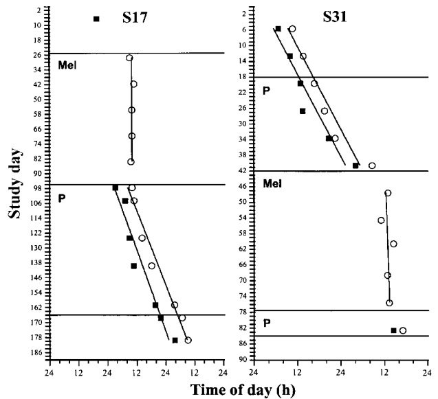
Figure 2 Acrophase times of the circadian phase markers for two subjects who entrained during melatonin treatment (S17, S31). Other details as in Fig. 1.
